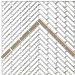
13 PIECES M 2 8x32,5cm - 3.1"x12.8" 48 6x24,5 cm - 2.4"x9.6" 68
