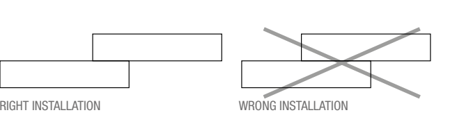
RIGHT INSTALLATION
